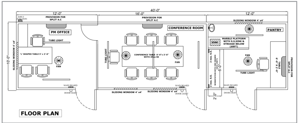
Portable Office
