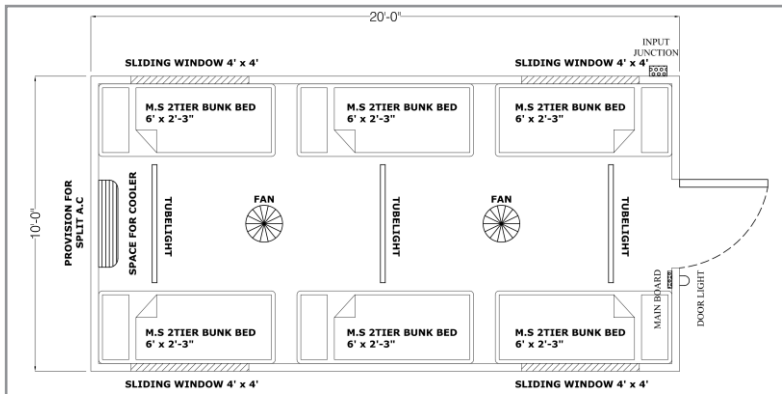
Portable Accomodation
